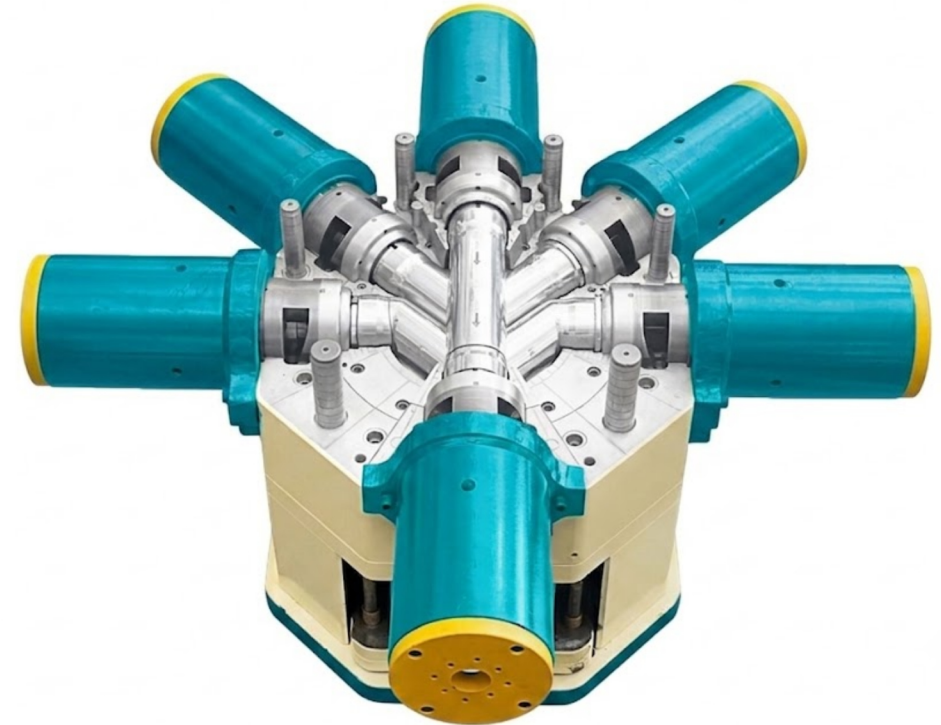
Inspection Chamber 6-Way Mould
