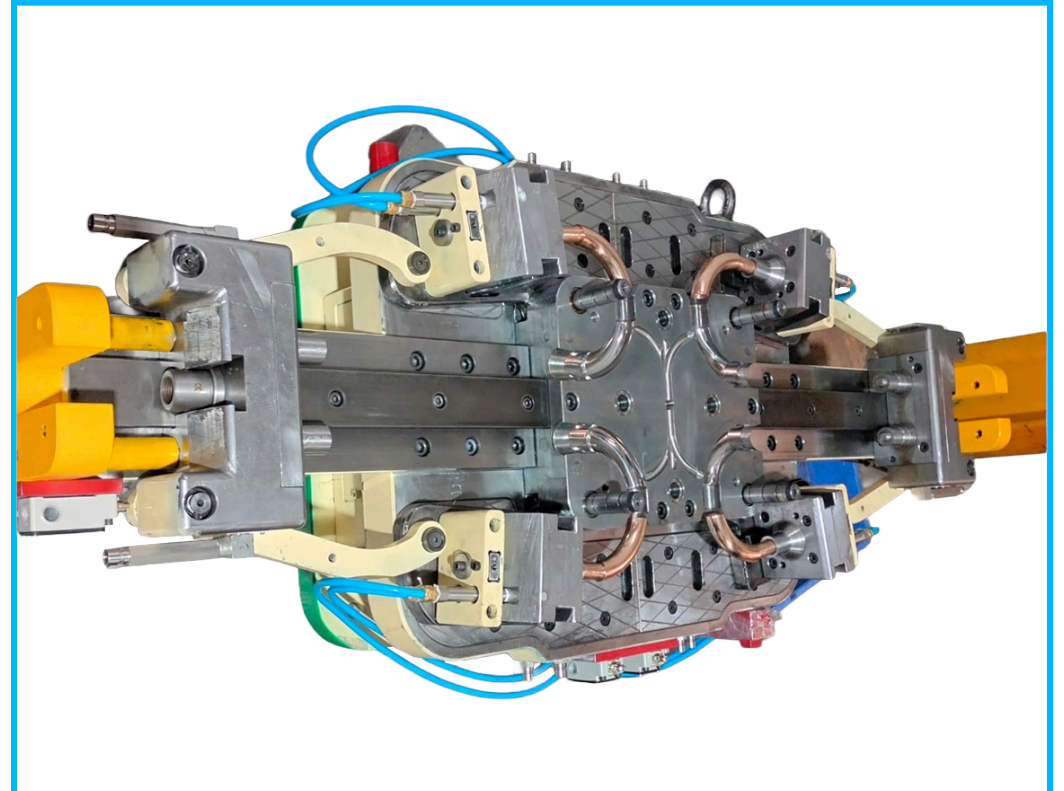
Sweep Bend Mould
