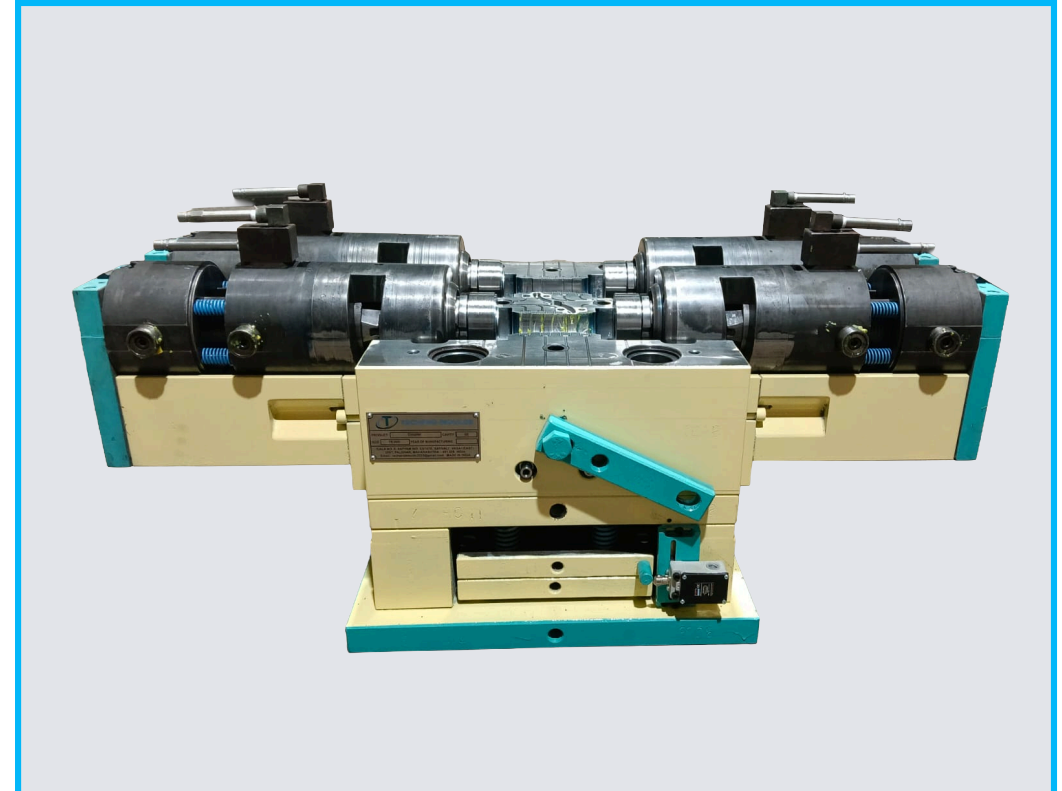
SWR Collapsible Coupler Mould
